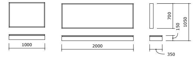
DORA™ Vanity WALL SET
