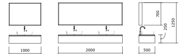
KATE™ WASH STAND WALL SET
