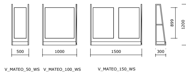
MATEO™ Vanity WALL SET
